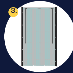
Frameless PV Module with special glued profiles on the back face is attached on the hooks.
